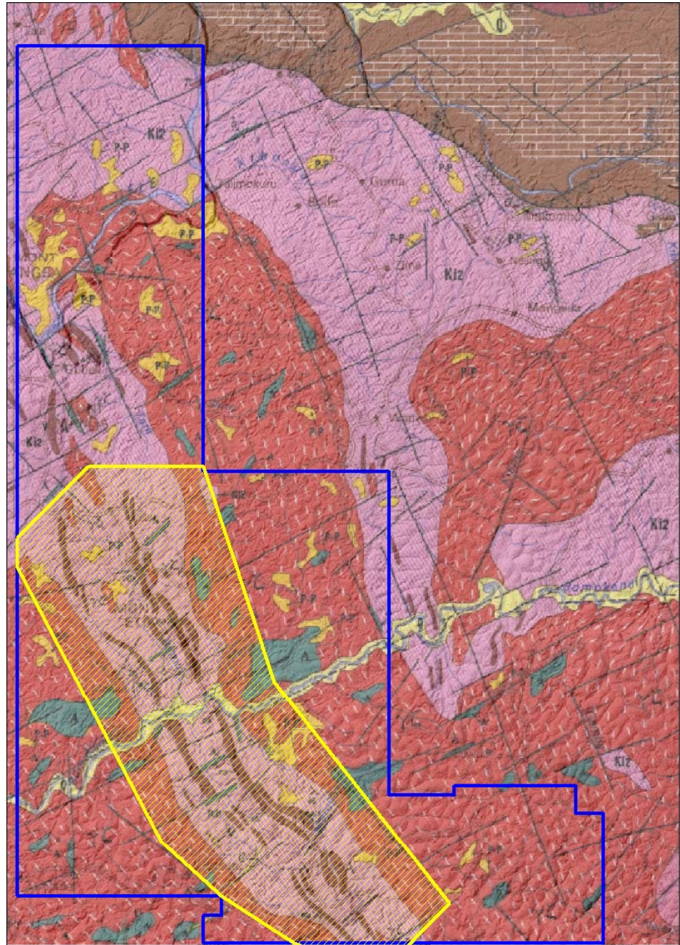
1:500,000 Geology over SRTM
